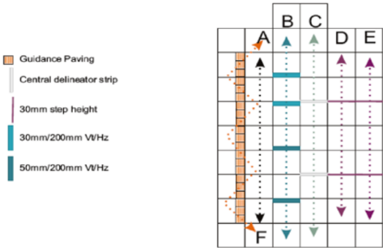
Figure 3: Layout of delineators for mobility impaired participants
