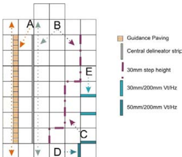
Figure 2: The layout of delineators on the platform for blind and partially sighted participants
